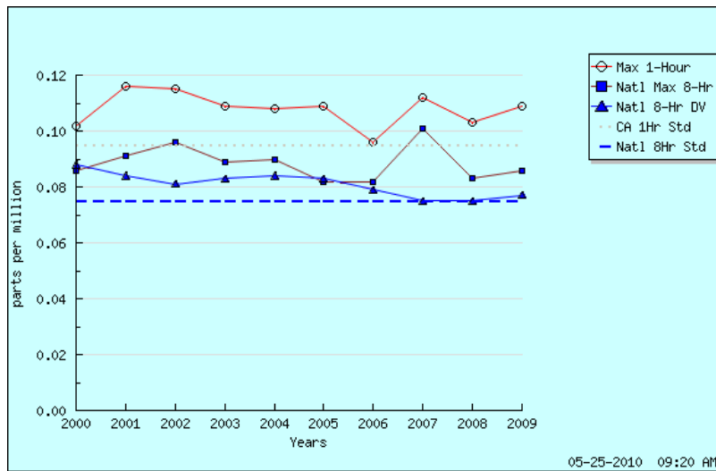
Figure 7 Ozone Trends Summary: Thousand Oaks-Moorpark Road
