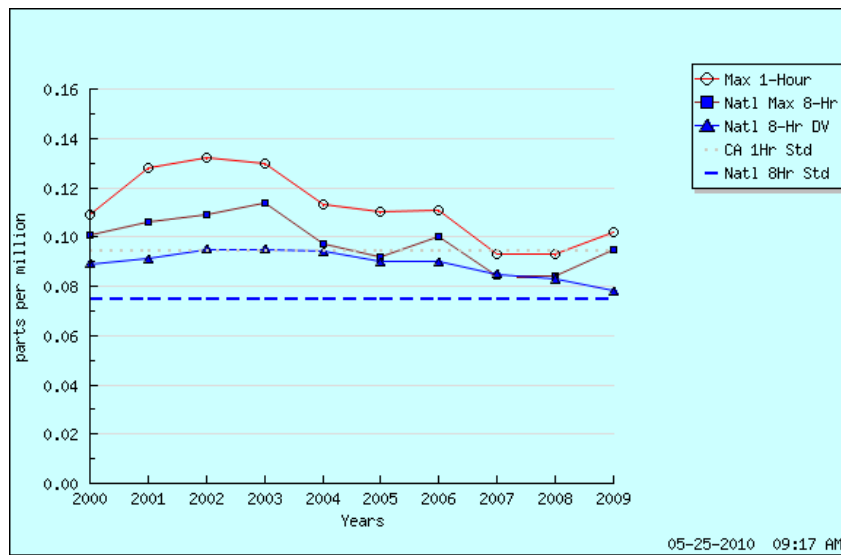
Figure 4 Ozone Trends Summary: Ojai-Ojai Avenue
