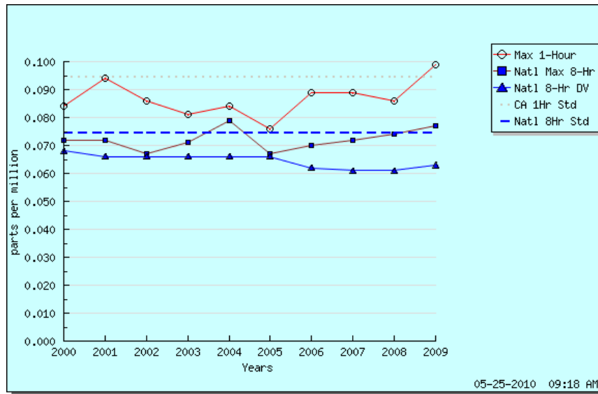
Figure 3 Ozone Trends Summary: El Rio-Rio Mesa School #2
