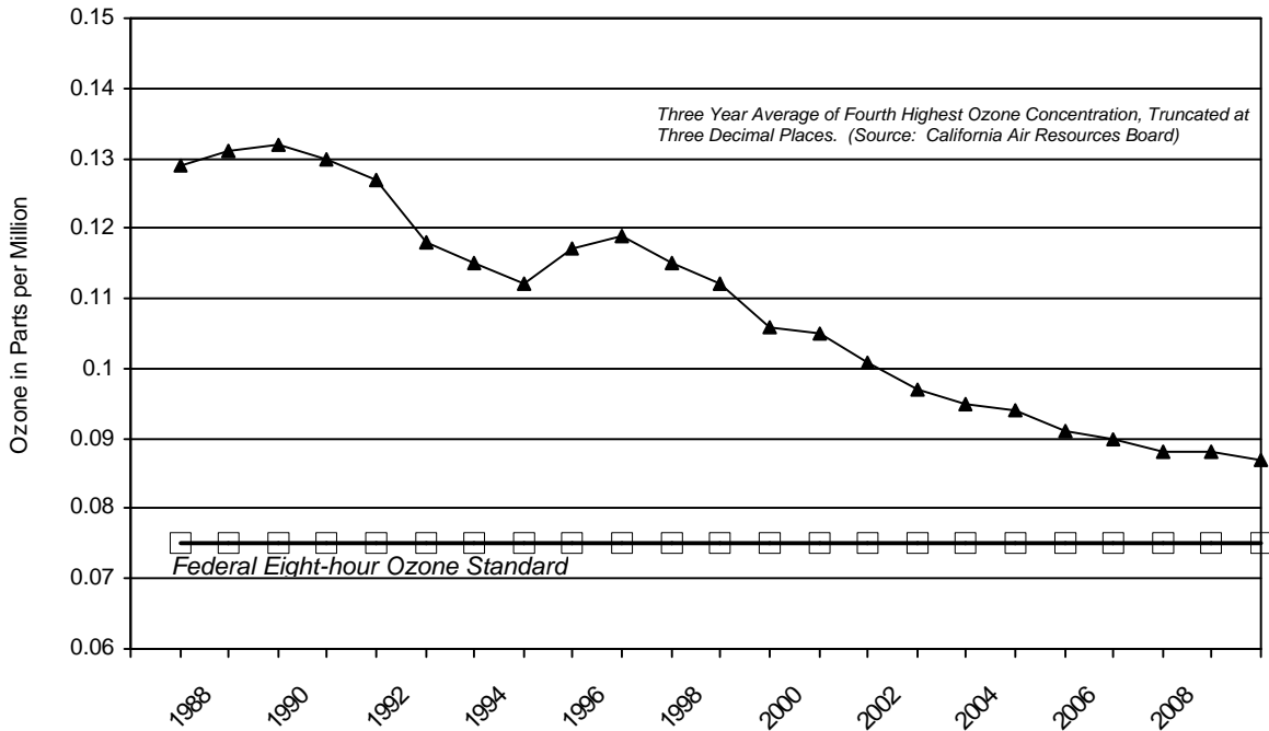
Figure 2 Historical Eight-Hour Ozone Trends Three Year Average of Fourth Highest Concentration
