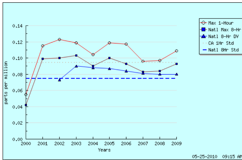
Figure 5 Ozone Trends Summary: Piru-3301 Pacific Avenue
