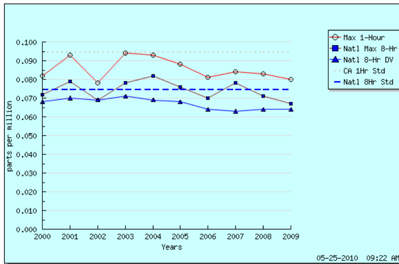
Figure 8 Ozone Trends Summary: Ventura-Emma Wood State Beach
