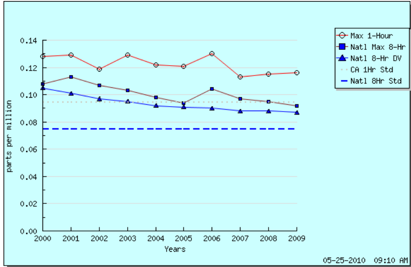
Figure 6 Ozone Trends Summary: Simi Valley-Cochran Street
